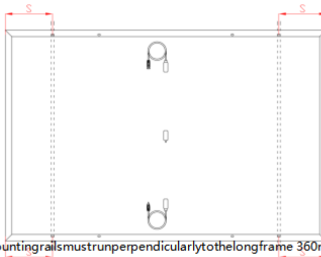
Figure12-1:Mountingrails mustrunperpendicularto thelongframe 360\text{mm} < S < 410\text{mm}
