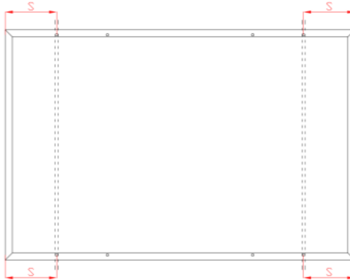
Figure12-1:Mountingrails mustrunperpendicularto thelongframe 360\text{mm} < S < 410\text{mm}
