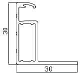
Section diagram of long frame profile
